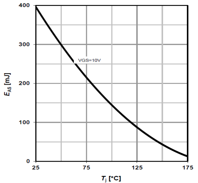
Avalanche energy
