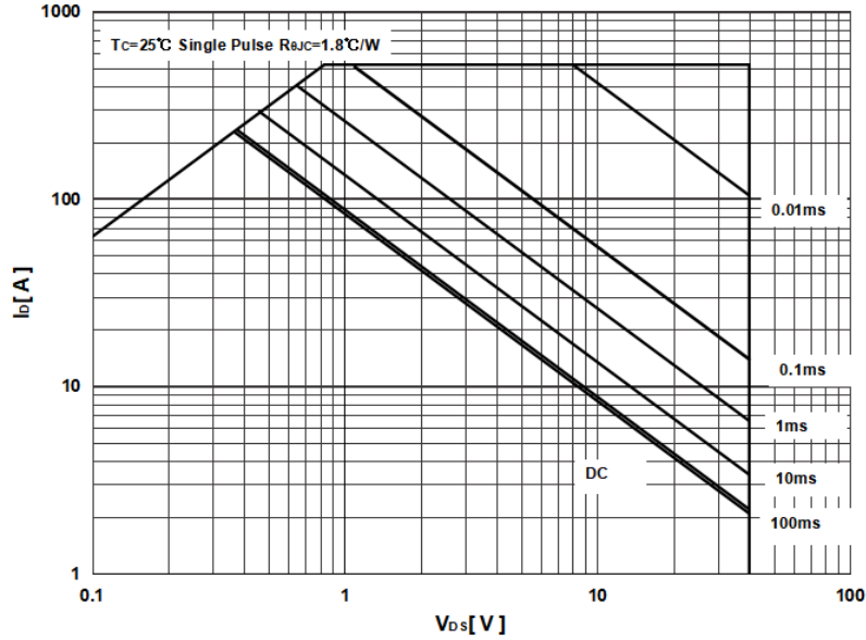
Maximum Forward Biased Safe Operating Area
