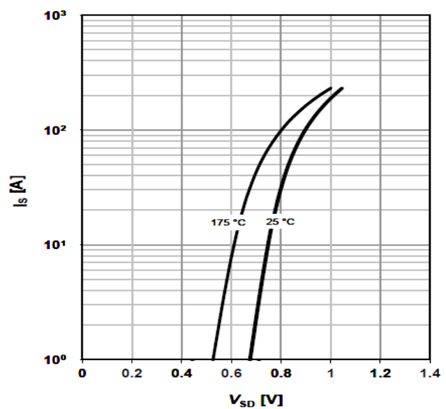
IS -- VSD
